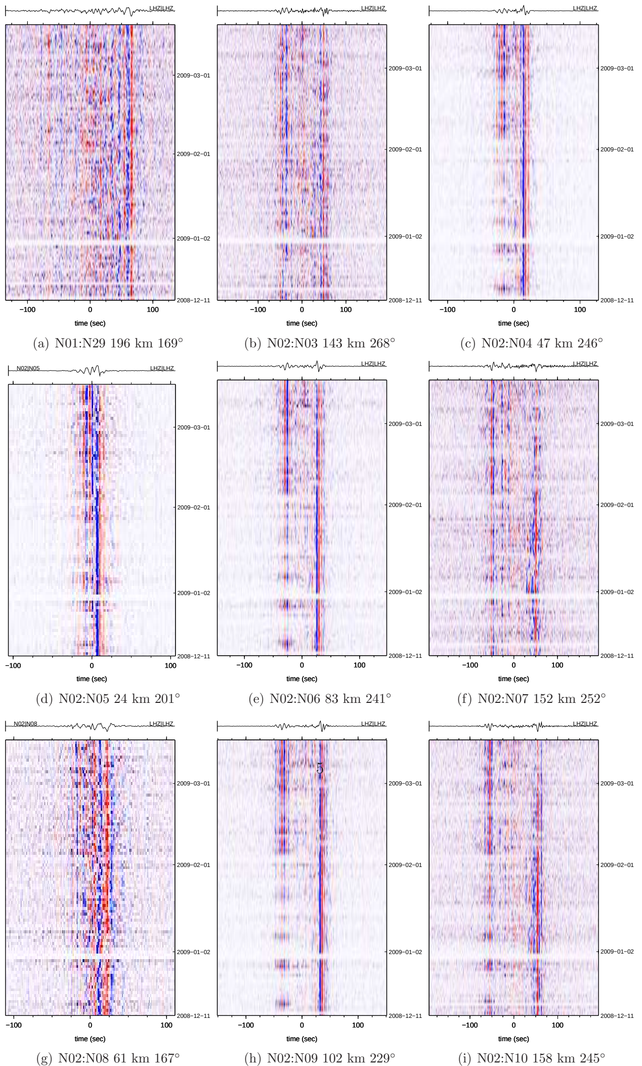
Figure 4: CREST ambient noise
