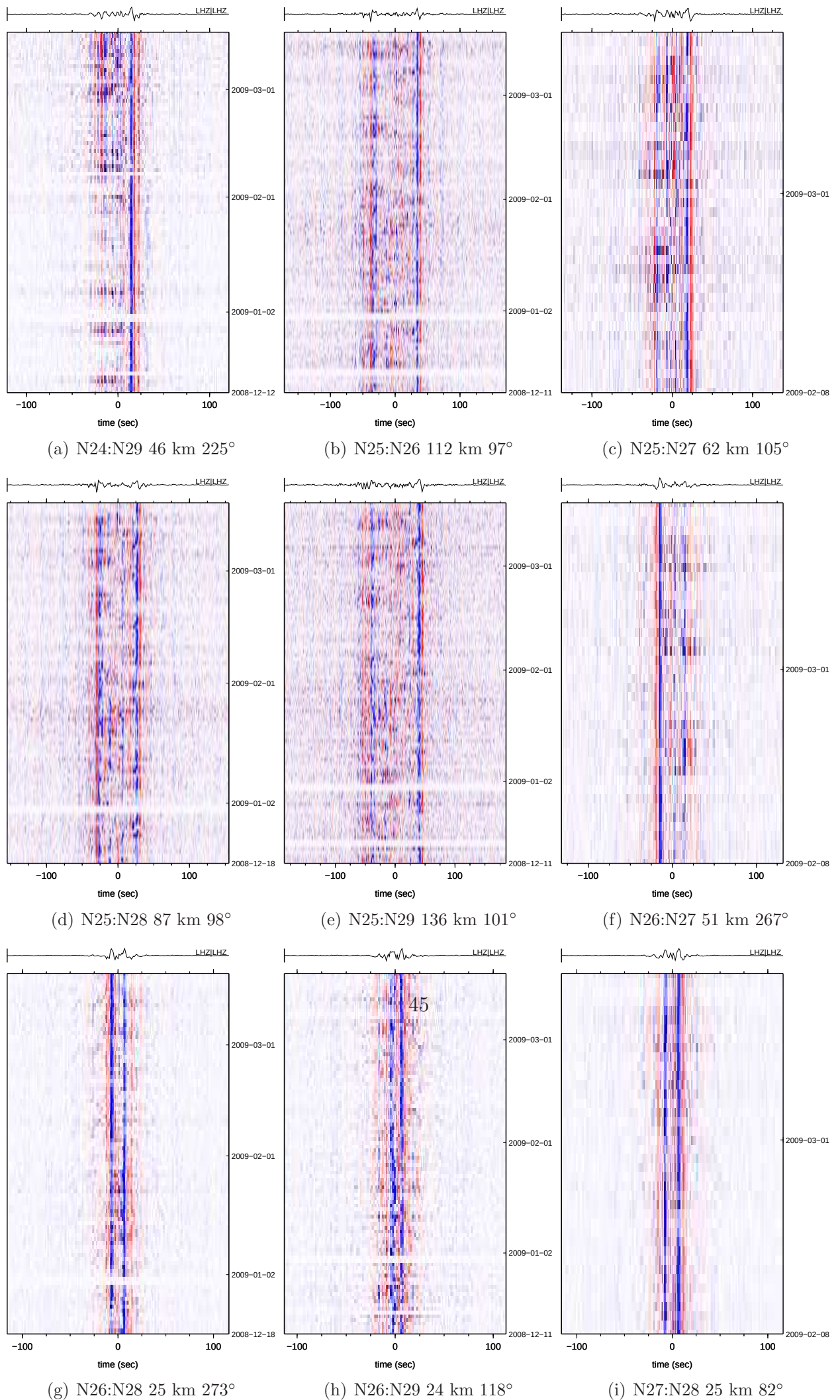
Figure 44: CREST ambient noise
