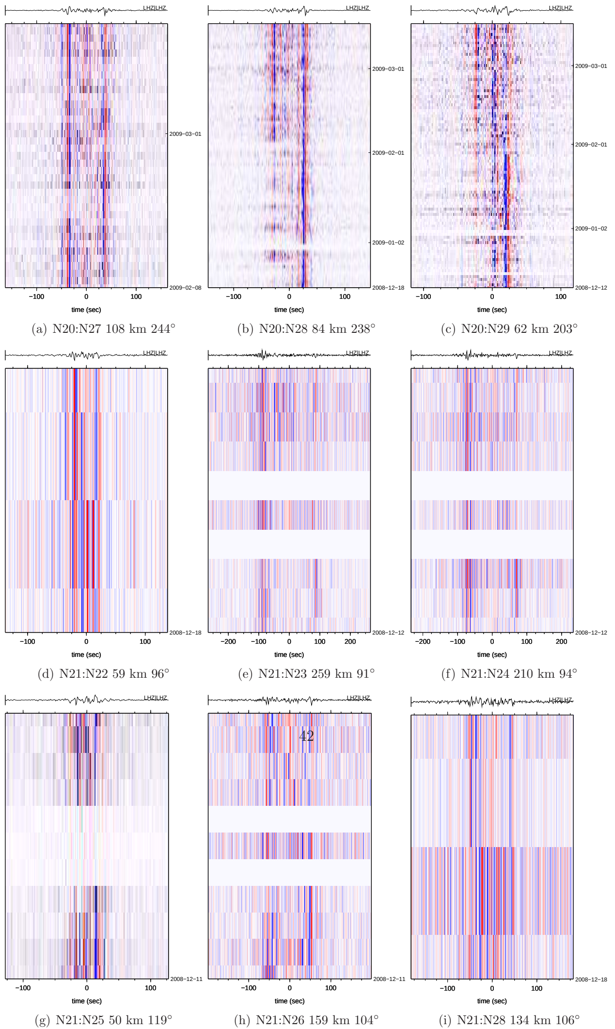
Figure 41: CREST ambient noise
