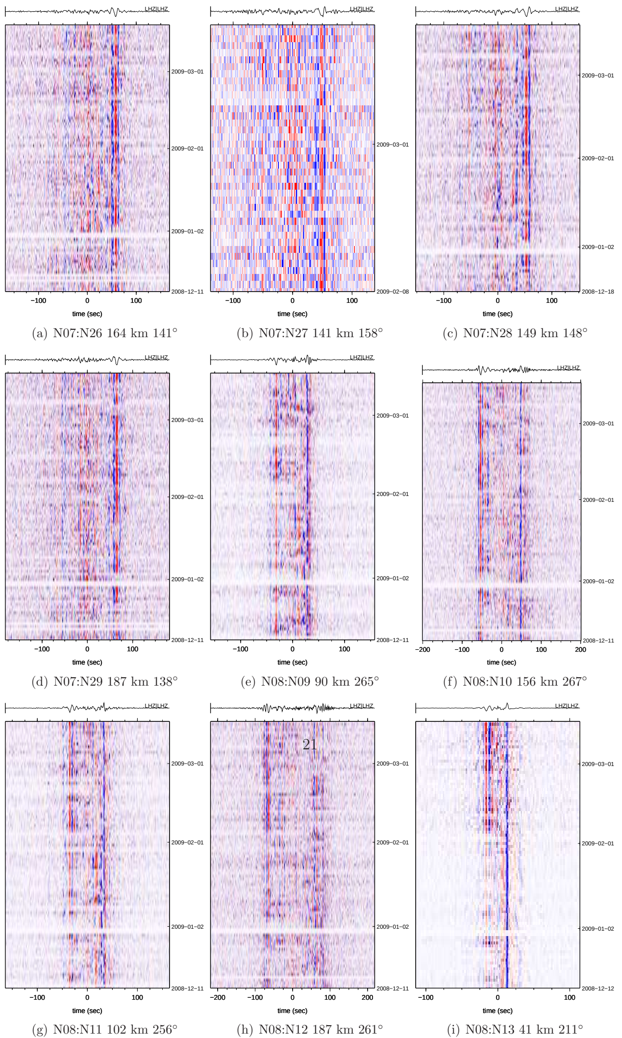
Figure 20: CREST ambient noise
