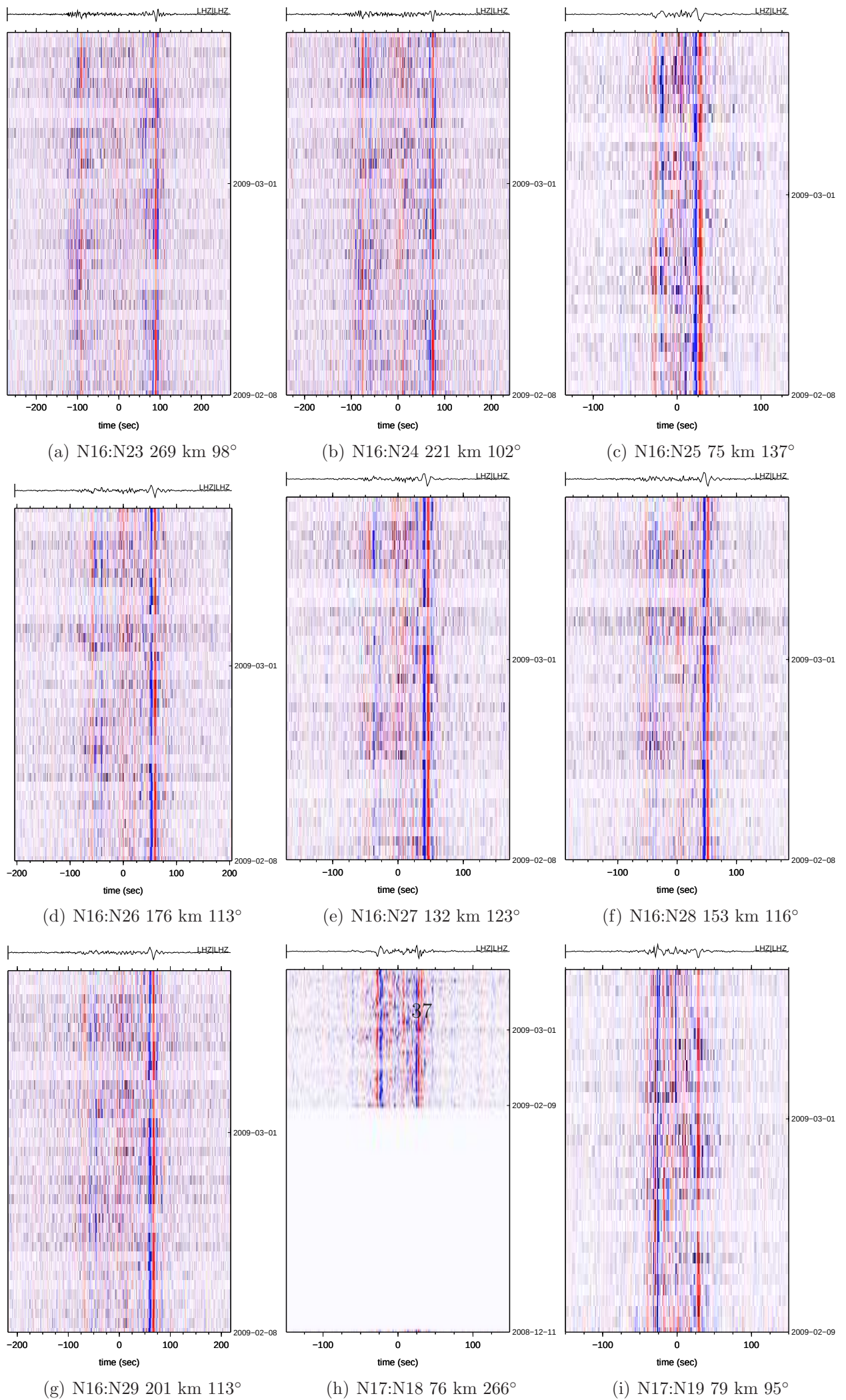
Figure 36: CREST ambient noise
