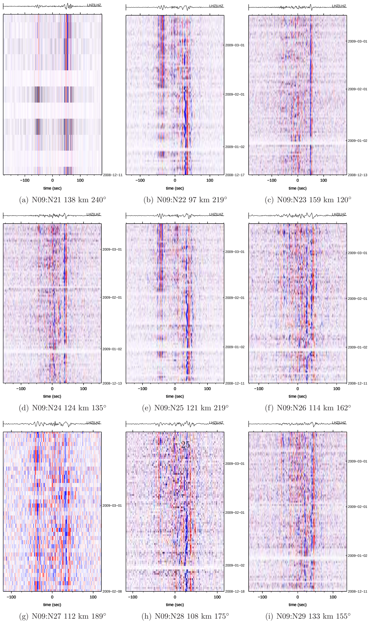
Figure 24: CREST ambient noise
