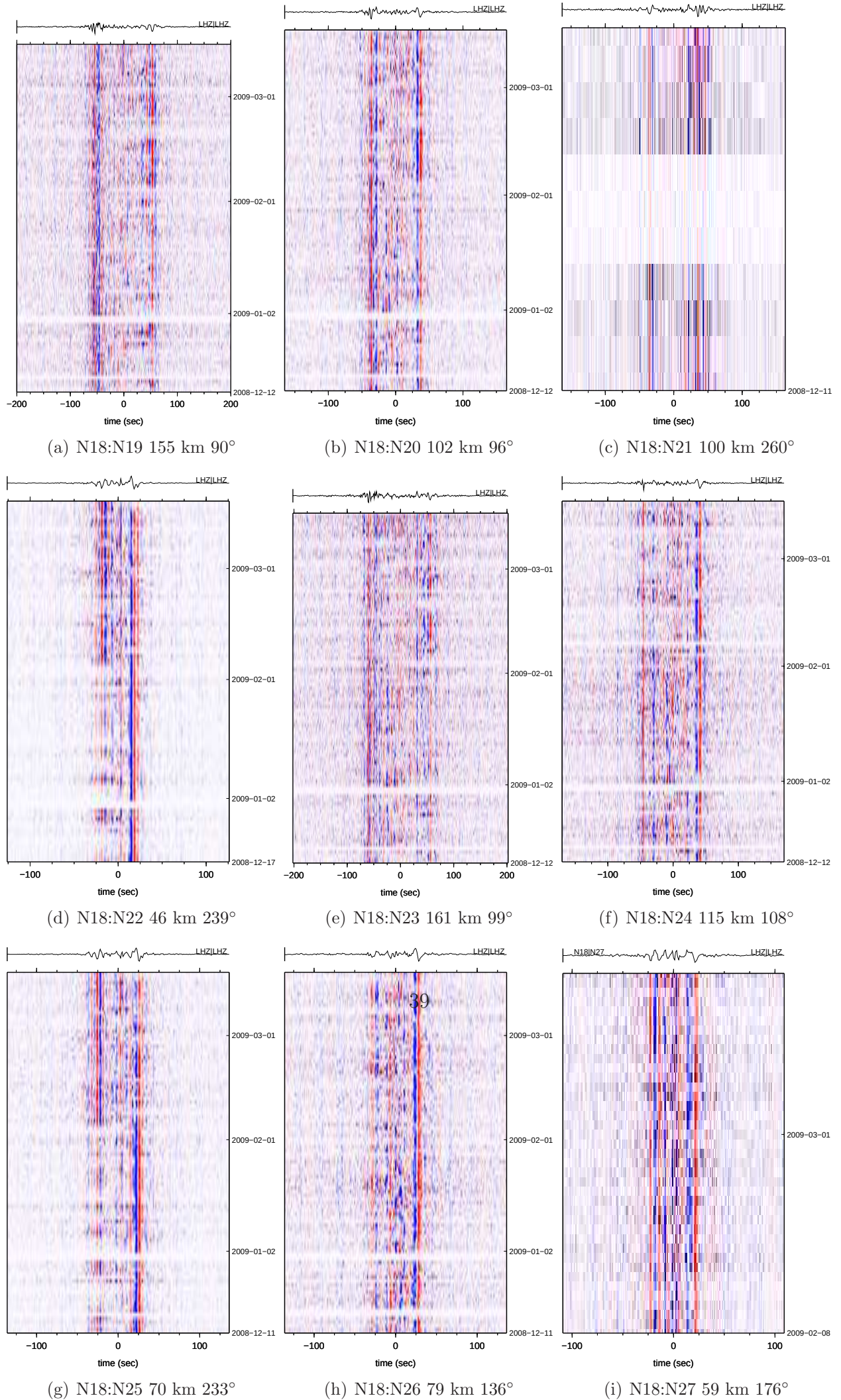
Figure 38: CREST ambient noise
