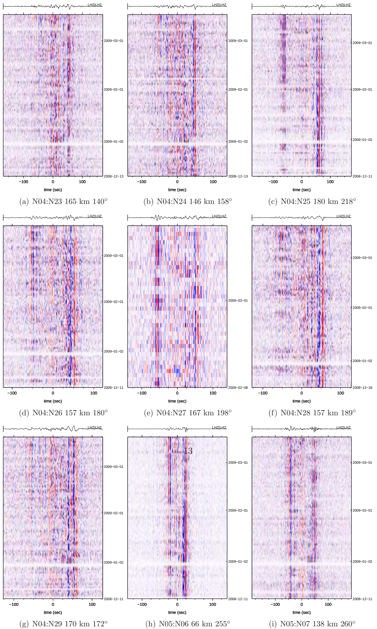
Figure 12: CREST ambient noise
