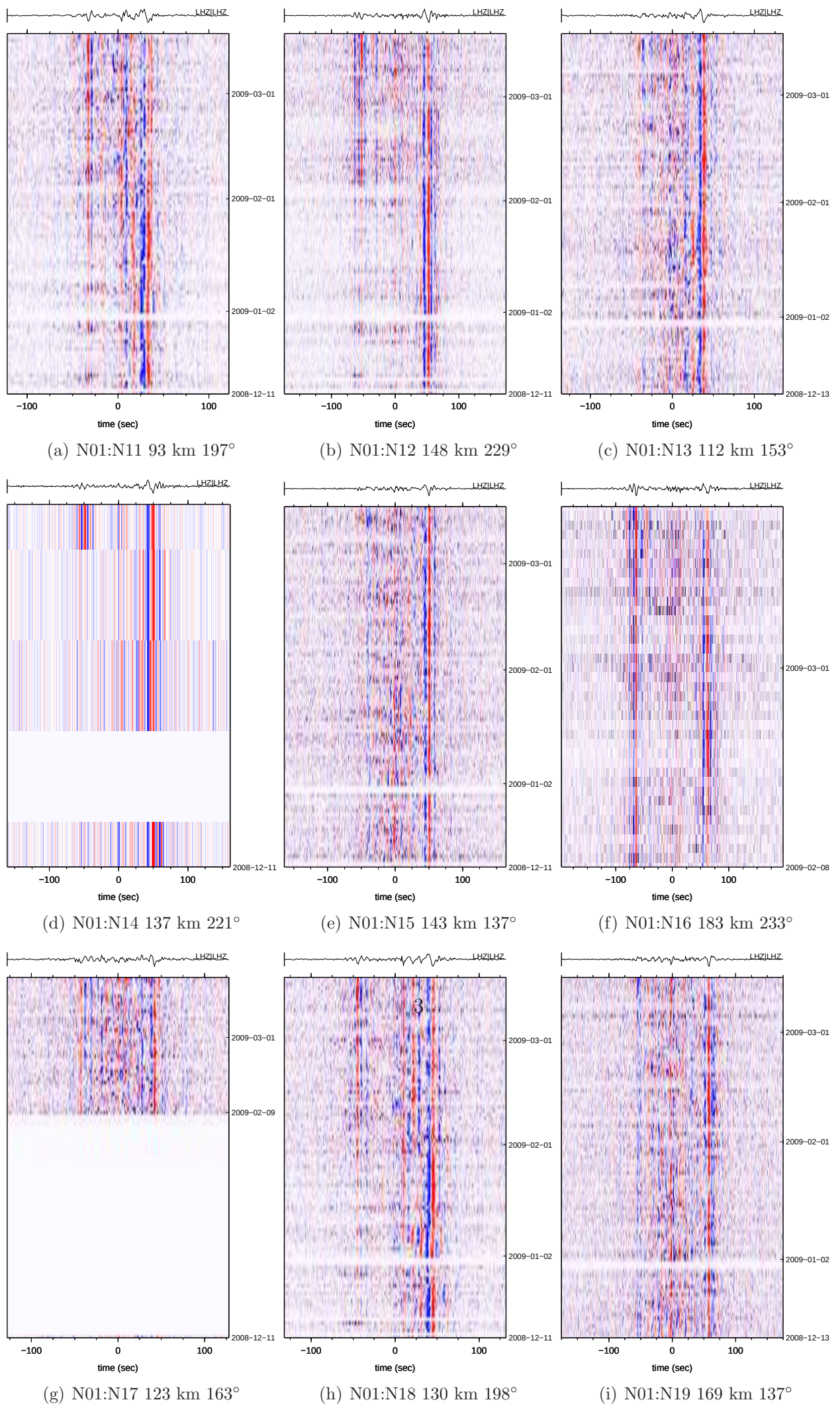
Figure 2: CREST ambient noise
