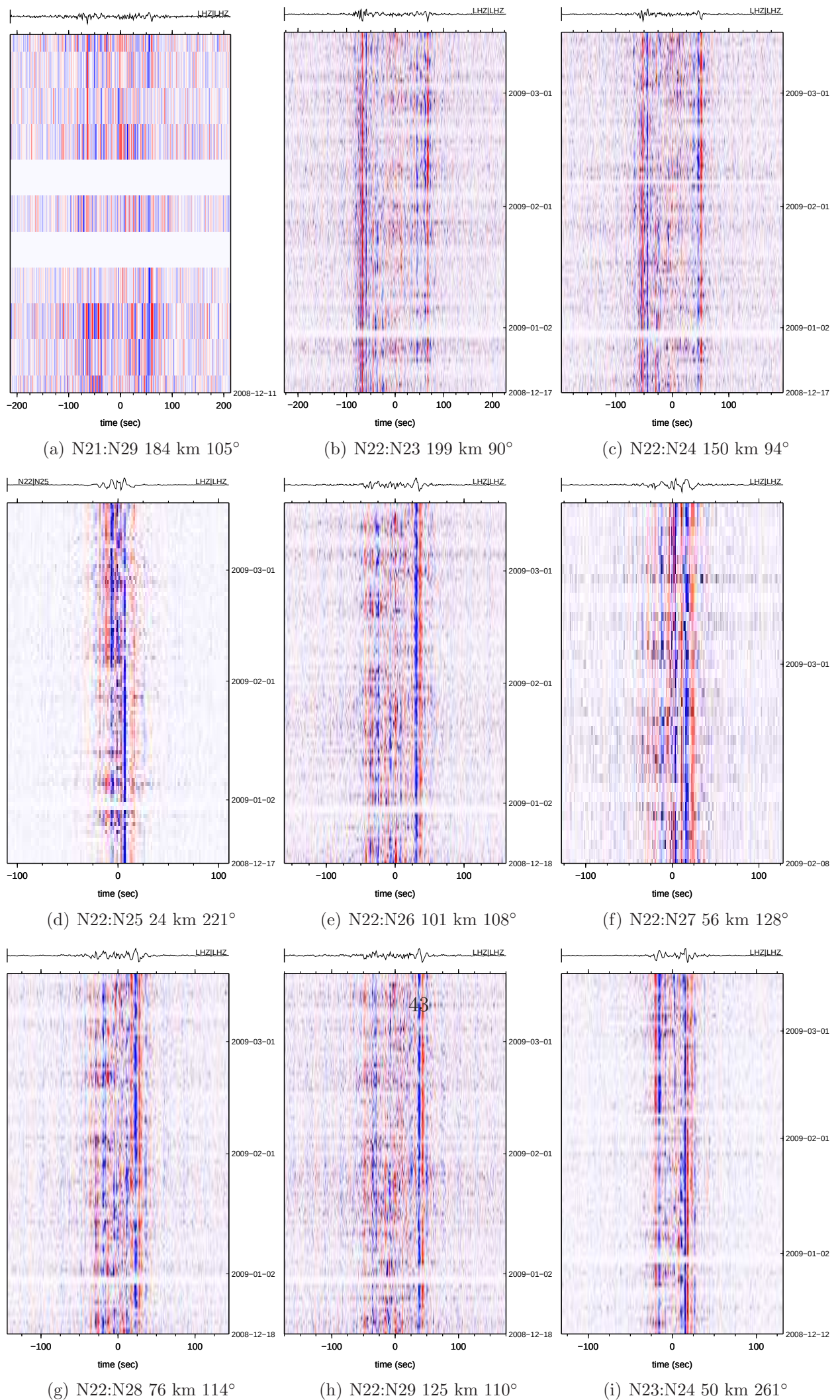
Figure 42: CREST ambient noise
